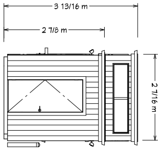
E4 EAST EXTERIOR ELEVATION scale: 1:50
