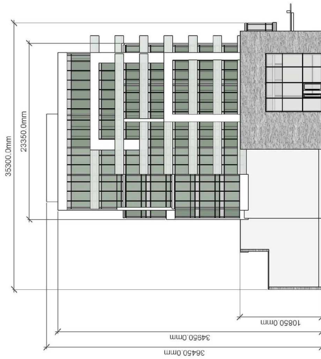
BUILDING B NORTH ELEVATION
