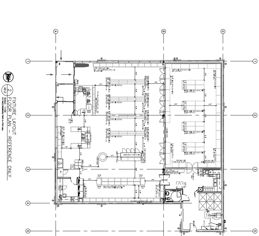
1 INTERIOR FIT UP FLOOR PLAN - REFERENCE ONLY 2 FIXTURE LAYOUT FLOOR PLAN - REFERENCE ONLY
