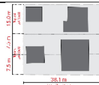
Typical Lot Dimensions
