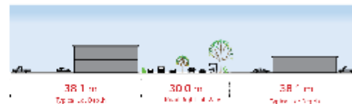
Typical Cross Section – A-A
