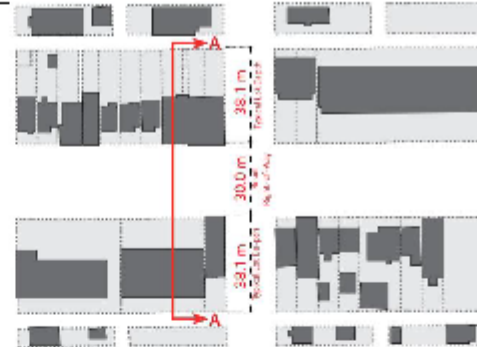
Typical Block Pattern
